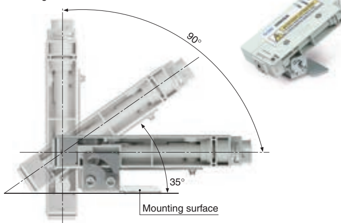
Pivoting bracket
